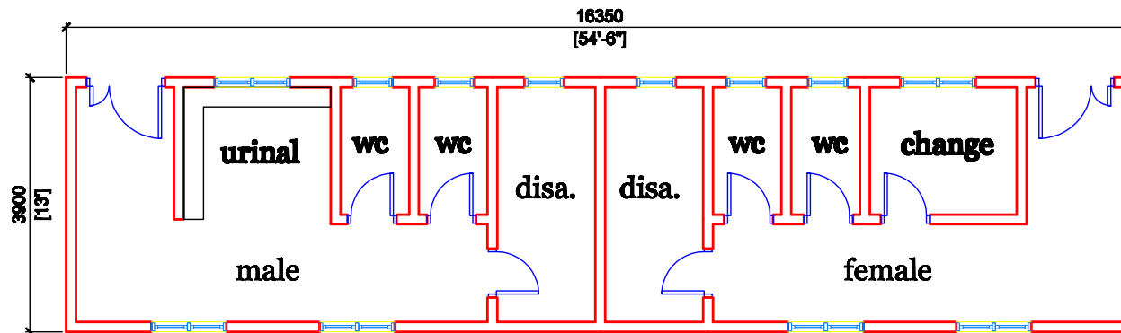
6-SEATER TOILET FOR EWUSIEJOE M/A GIRLS MODEL SCHOOL
